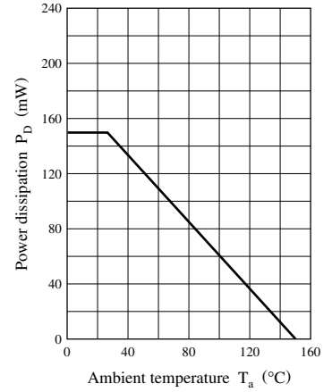
P_D - T_a
